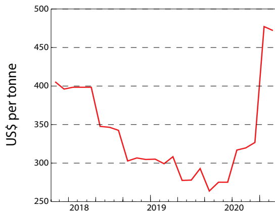
Chart 3.1 Methanol
